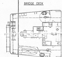
BRIDGE DECK
