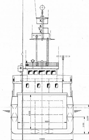
MIDSHIP SECTION
